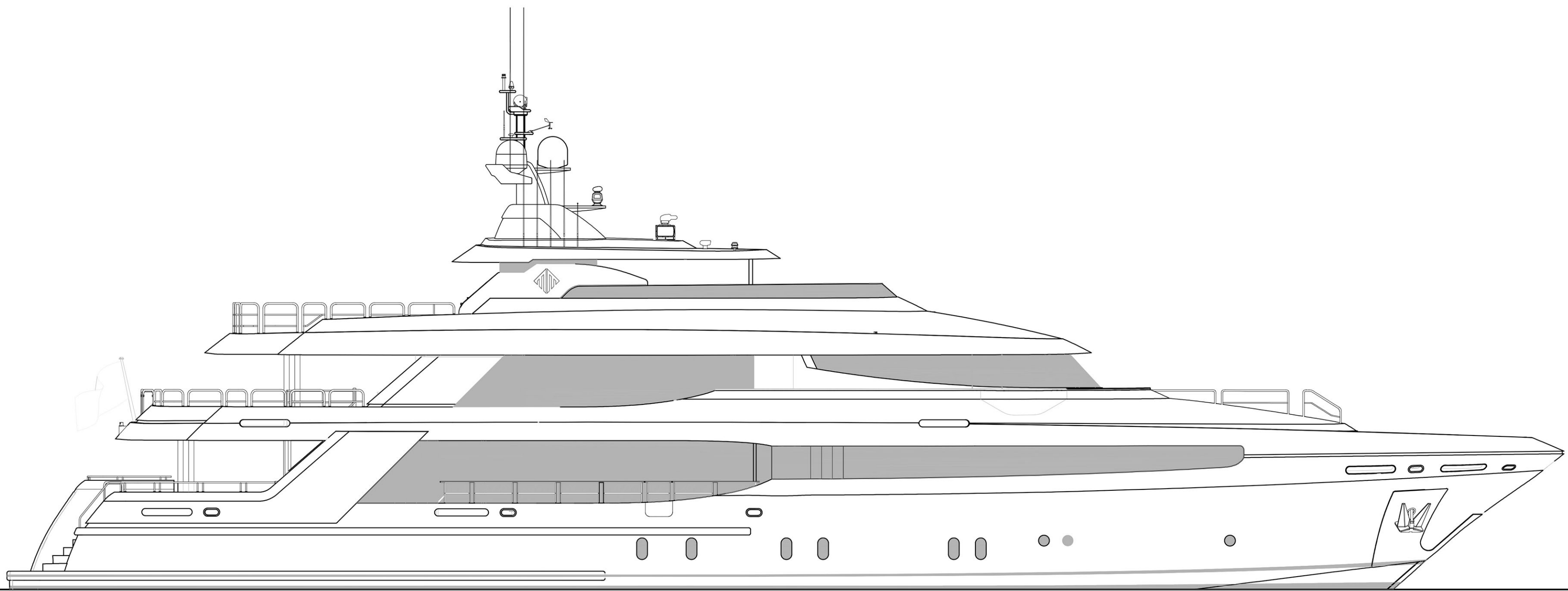
PROFILE
